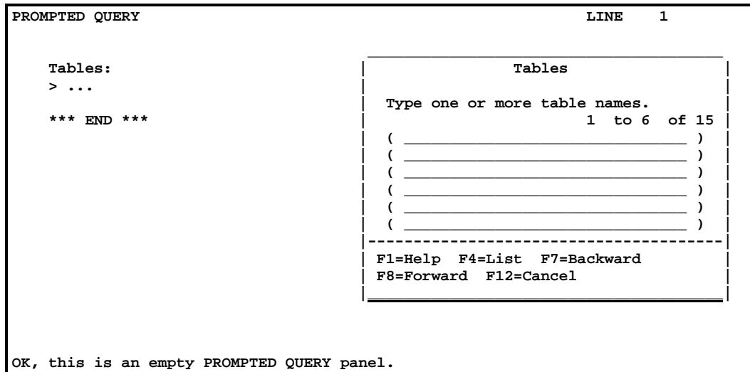
Figure 5–29, Prompted Query Panel
