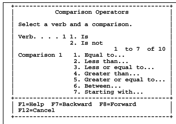
Figure 5–40, Comparison Operators Dialog Panel
