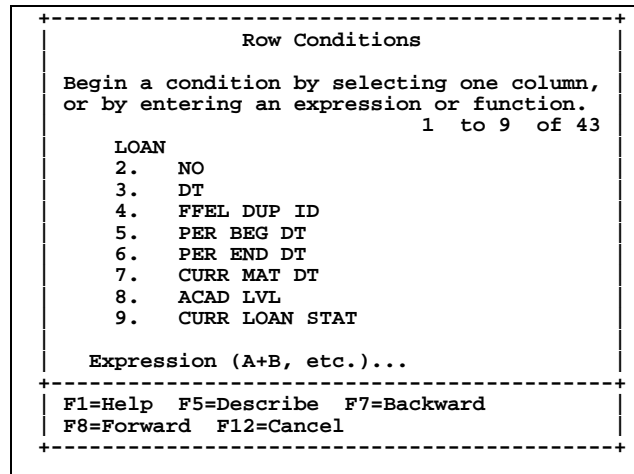
Figure 5–39, Row Conditions Dialog Box
