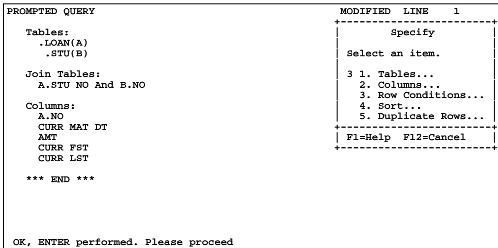
Figure 5-53, Columns Selected Displayed in Echo Area
