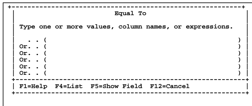
Figure 5–42, Equal To Dialog Panel
