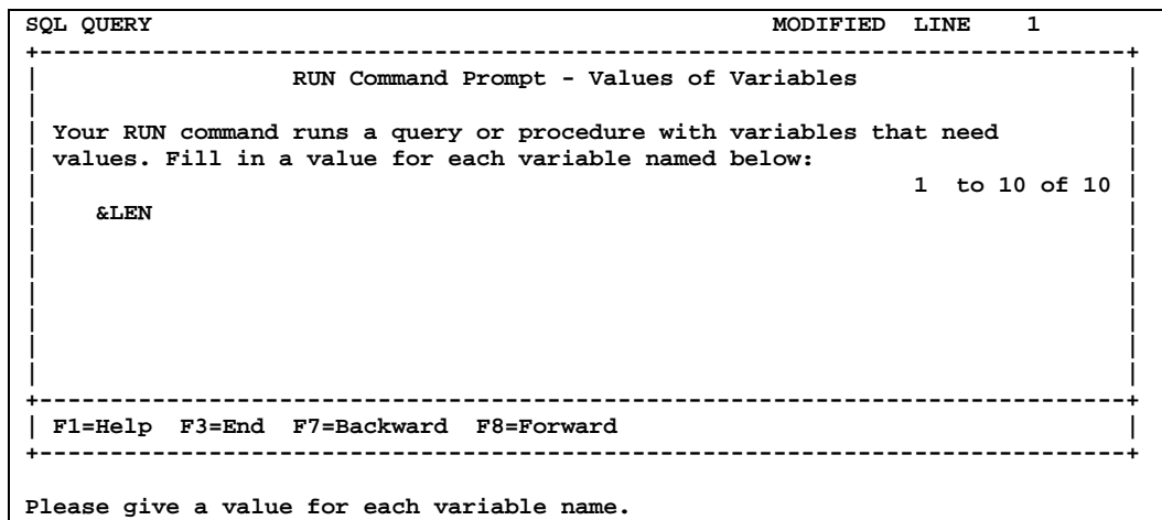
Figure 5–91, RUN Command Prompt Panel
