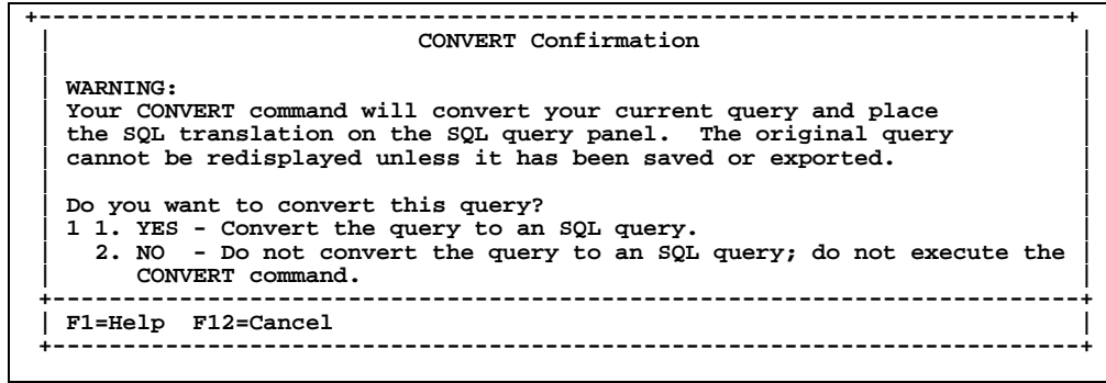
Figure 5-48, Convert Confirmation Panel
